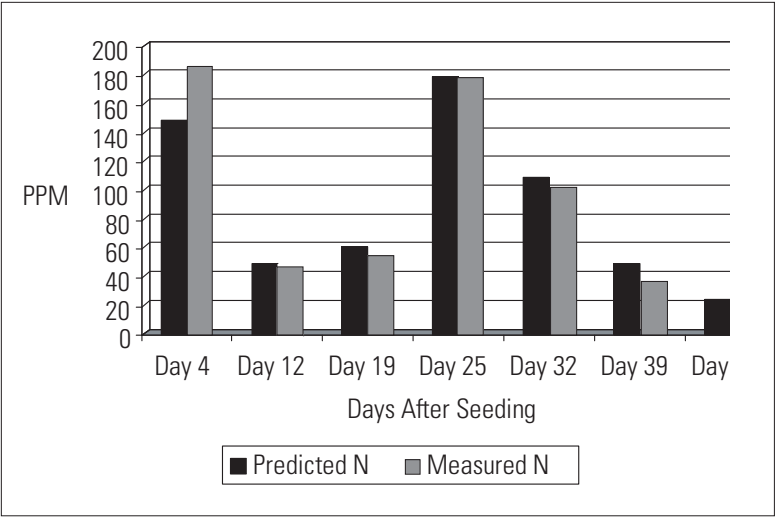
Figure 4-8. A comparison of predicted (based on conductivity) and measured nitrogen concentrations in a float bed, 2002
